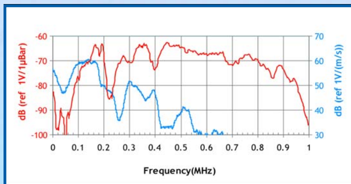
Frequency response of the R50α. Calibration based on ASTM E1106; Calibration based on ASTM E976.
